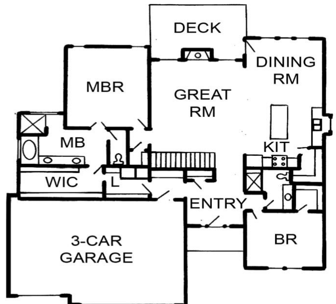
Main Floor Garage
